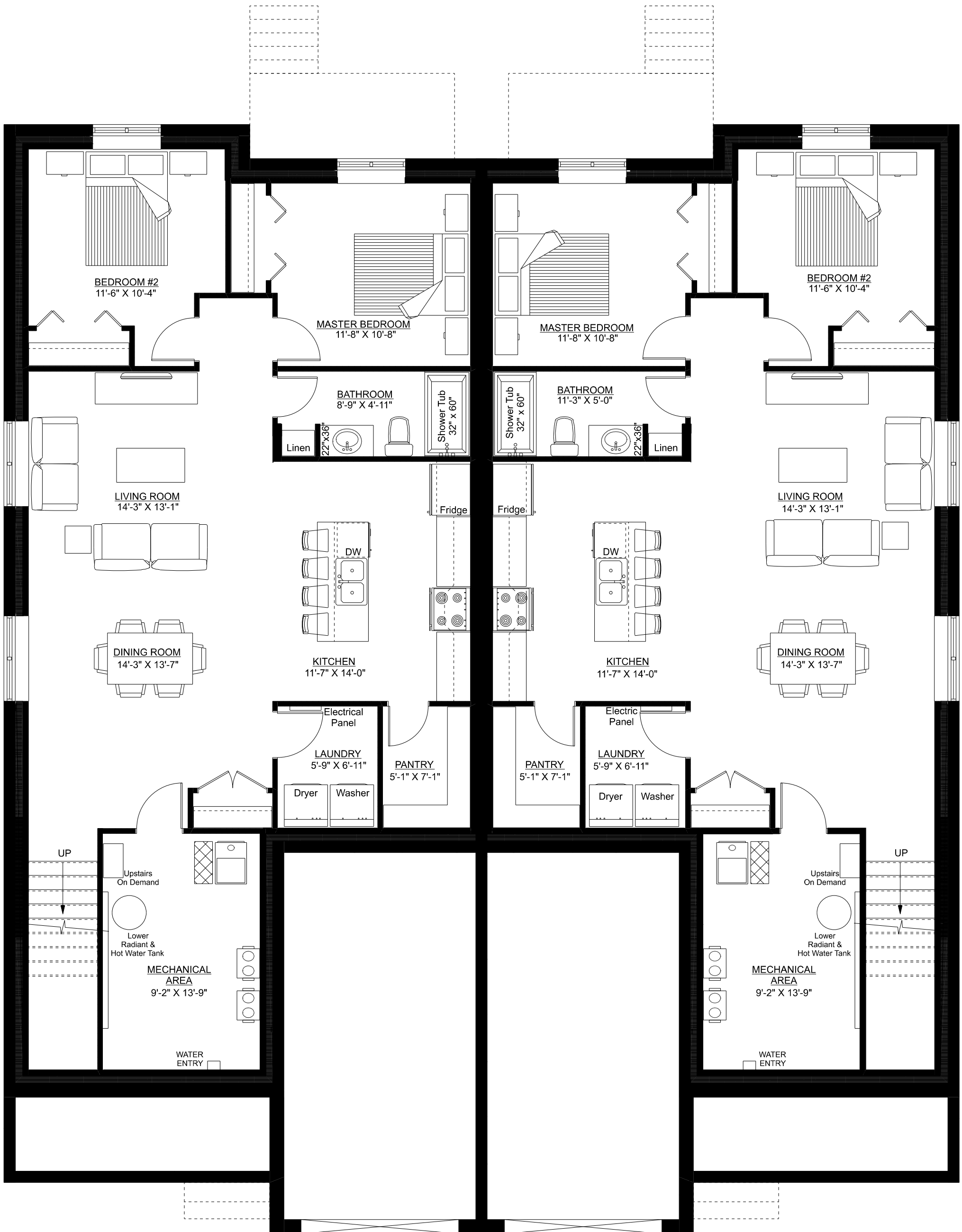
BASEMENT FLOOR PLAN
